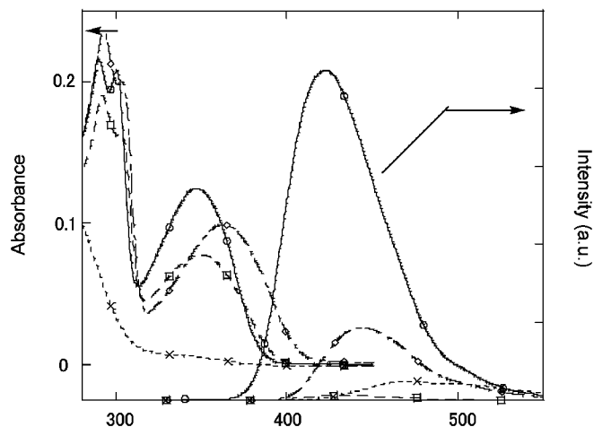
Figure 3. Absorption and Fluorescence Spectra of 6 (O), 8 (◇), 9 (□), and 10 (x) in Methanol. [ 6 ] = [ 8 ] = [ 9 ] = [ 10 ] = 1 \times 10^{-5} M, Excitation Wavelength; 289.5 nm ( 6 ), 293.5 nm ( 8 ), 292.5 nm ( 9 ), and 248.5 nm ( 10 ).
